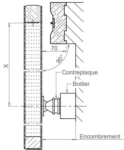
Bloc-Porte Double Action
